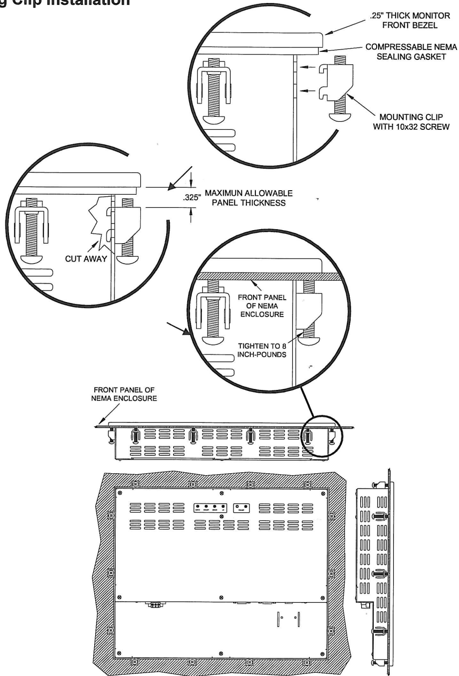
REAR VIEW OF PANEL MOUNTED UNIT
